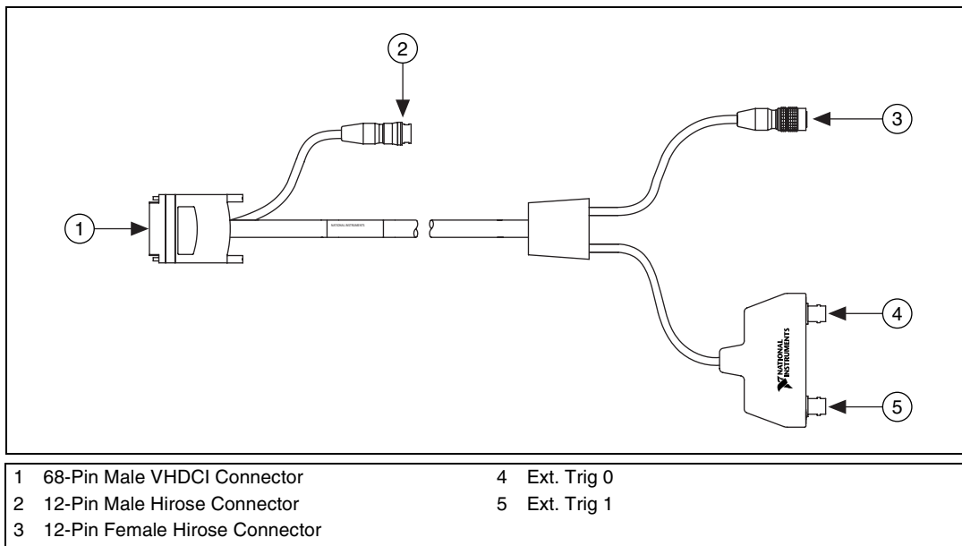
Figure 1. IMAQ A8055 Cable
